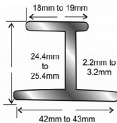
Outer Frame For Windows
