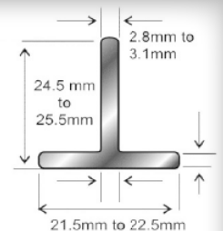
Vertical And Horizontal Glazing Bar For Windows
